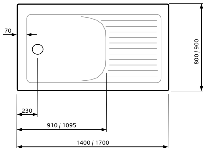
Rectangular Walk In (Curved Drying Area)
