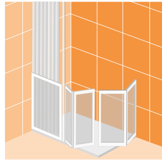
Option E 400mm fixed half height panel with floor to ceiling pole and a pair of bi-fold door meeting on corner
